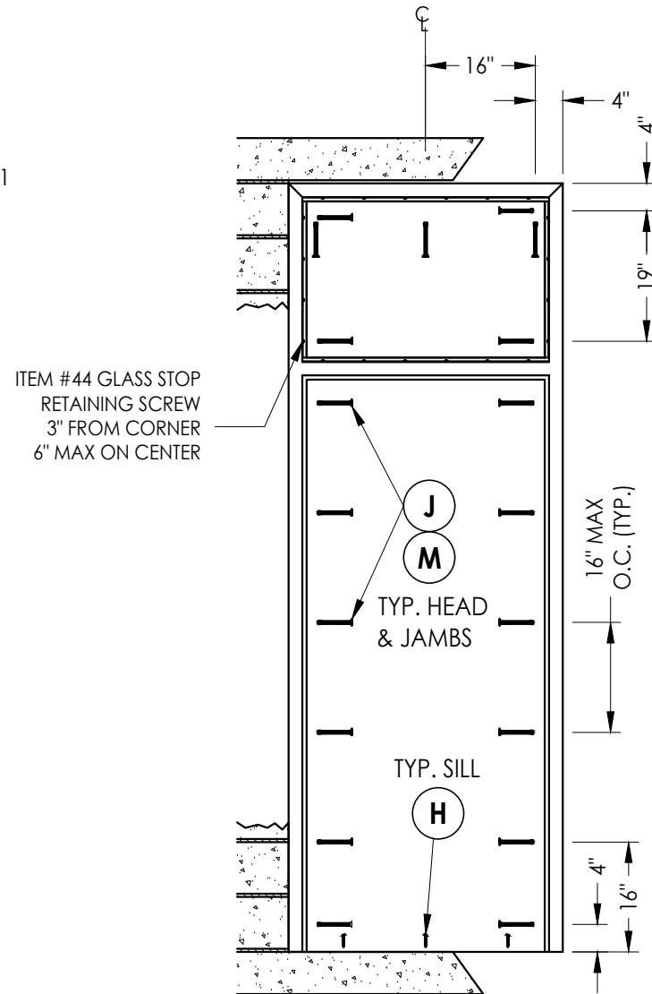
FRAME ANCHORING
