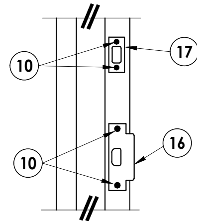
DETAIL 2
